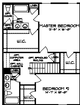
2ND FLOOR PLAN W/ STD. 2 BEDROOM
