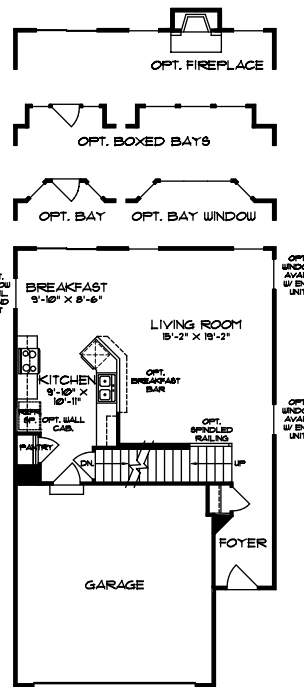
1ST FLOOR PLAN W/ STANDARD 2 BEDROOM
